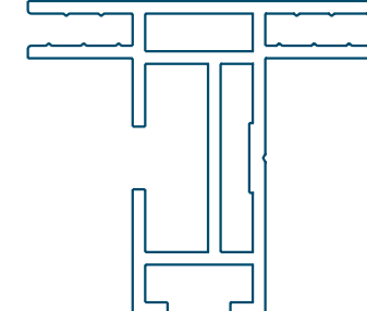
FitFRAME duo50 compact 29.0549.31
