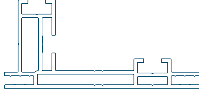
FitFRAME lightbox 100 29.0100.31
