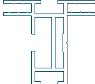
FitFRAME duo50 29.0649.31
