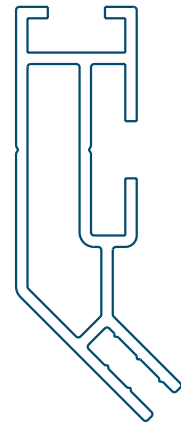
FitFRAME heavy 45° 29.4544.31
