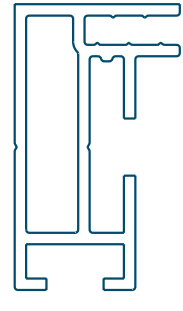
FitFRAME heavy 29.0644.31
