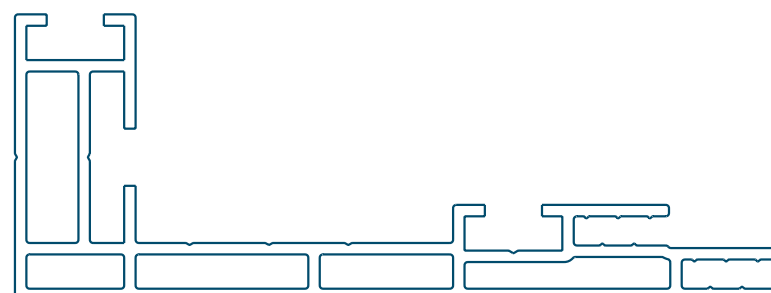
FitFRAME lightbox 120 29.0120.31
