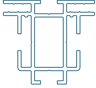
FitFRAME duo50S 29.3649.31
