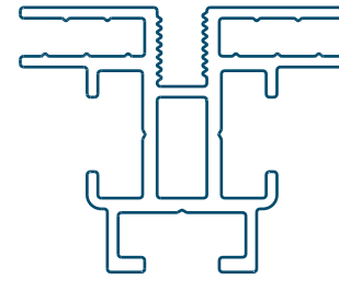
RAPit DOUBLE 40 31.2639.31
