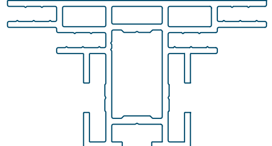
FitFRAME duo80 compact 29.0579.31
