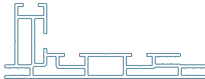
FitFRAME lightbox 120-2 29.0122.31
