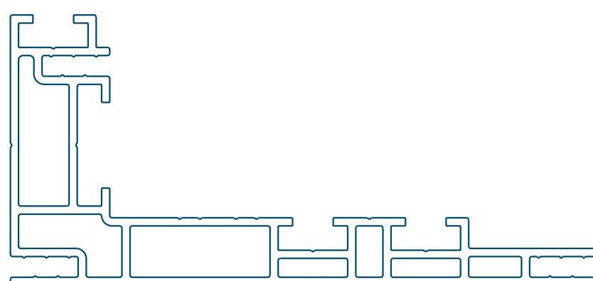
FitFRAME lightbox 130 29.0130.31
